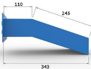
Stepped 285-335mm chute
