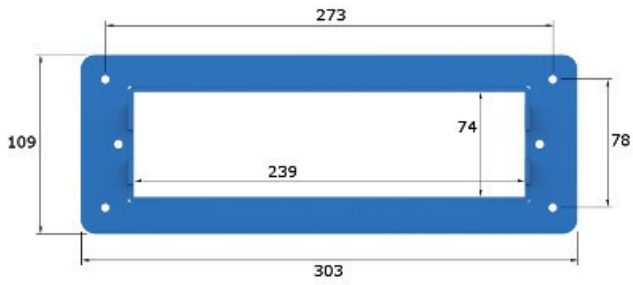
Flange for all chutes
