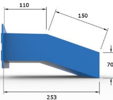
Stepped 195-245mm Chute
